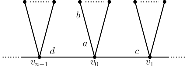
Figure 9: Configuration for the proof of Lemma 15, pre-coloured case.
