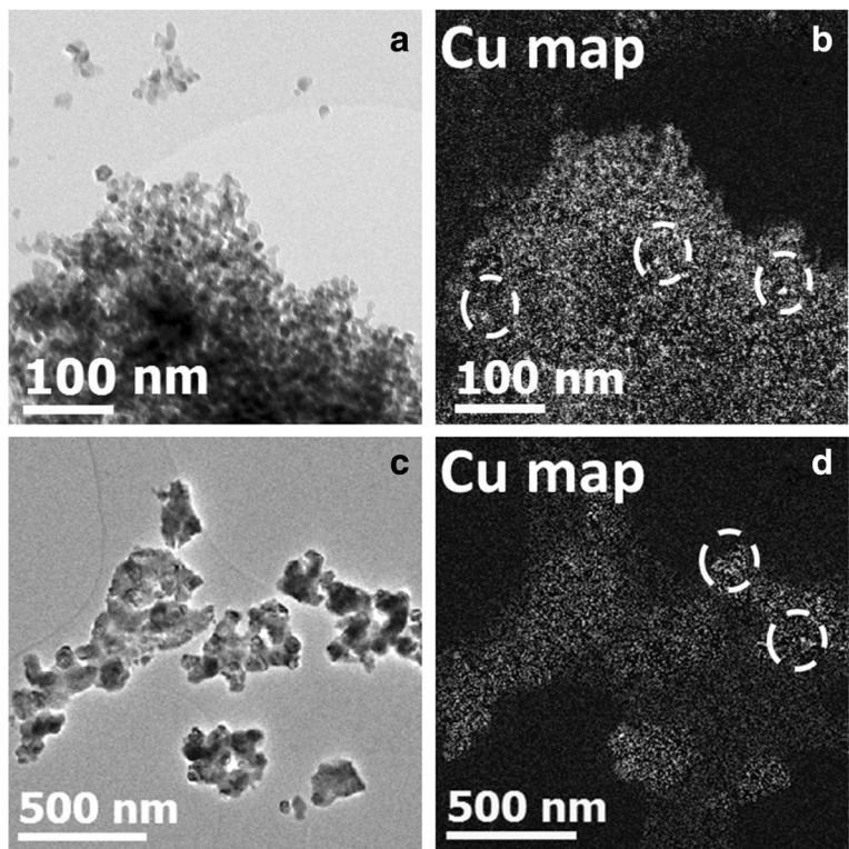
Fig. 5 Unfiltered images (a, c) and copper maps (EFTEM images) (b, d) using the Cu M threshold energy for Cu-8 samples calcinated at T_c = 600\text{ °C} (a, b) and at T_c = 900\text{ °C} (c, d)
