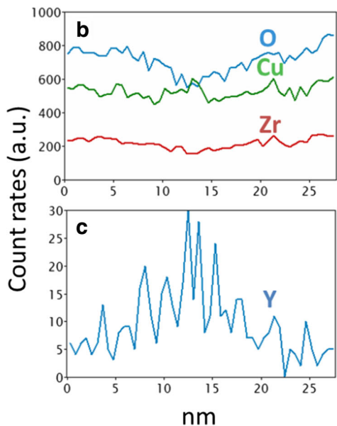
Fig. 6 a STEM HAADF image of Cu-8 powder calcinated at 900 °C. The dark regions with circular shapes in the grains correspond to the cavities. b, c EDX profiles across the grain boundary (red line in a) for O, Cu, and Zr (b) and Y (c) elements. A depletion of the number of counts for O, Cu, and Zr and an increase for Y is clearly seen
