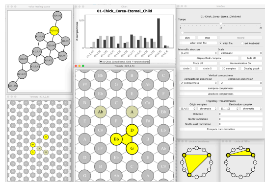
Fig. 1. Graphical User Interface of HexaChord.
