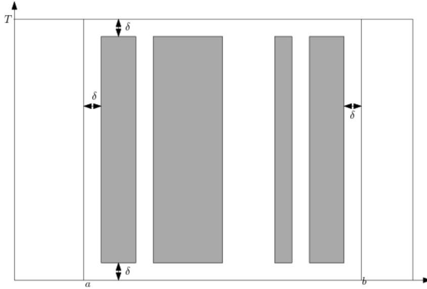
FIG. 4. An example of a \delta -covering set.
