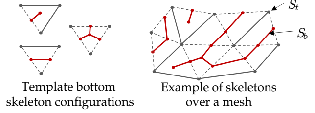
Fig. 8. Folds computation starts by choosing edges for the top skeleton S_t (gray) over a mesh \mathcal{M} (dotted gray) in the best fold direction. The bottom skeleton S_b (red) is deduced from S_t following the template (left)
