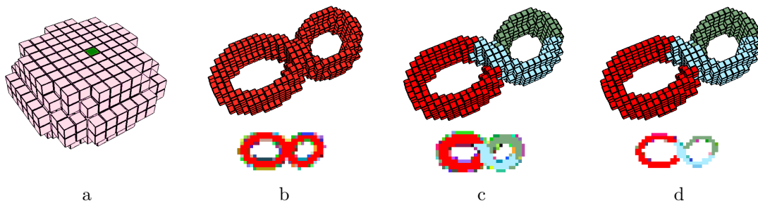
Figure 3: Experiments on 3D artificial images. The maximal value allowed on b_1 and b_2 is given for each images by Betti(b_1, b_2) . On the last three images, a slice of the image is provided to show the amount of different regions around the segmented part of the 2-torus. (a) Sphere with Betti(0,0) . (b) 2-torus with Betti(2,0) . (c) 2-torus with Betti(0,0) . (d) 2-torus with Betti(0,1) .
