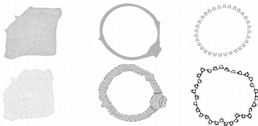
Figure 4. Layouts of crack (Left), fe_pwt (Middle) and finan512 (Right). (Top) Layouts obtained with FM 3 . (Bottom) Layouts obtained with MuGDAD
