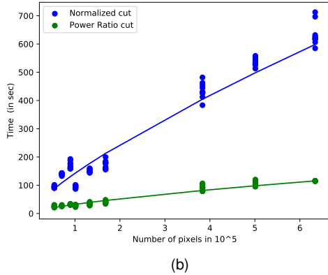
Fig. 11. (a) Scatter plot of the accuracy of normalized cuts vs power ratio cuts on hyperspectral data. The red line indicates the line x = y . As one can see, all the points lie above or on the line x = y . Hence power ratio cut results are better than normalized cuts (or at least equal). (b) Plots of executing times vs the number of pixels in the image. It is easy to observe that PRcut scales much better compared to normalized cuts.
