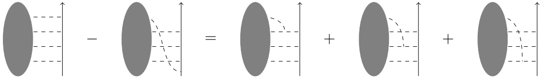
Figure 15: Recovering the link relation.
