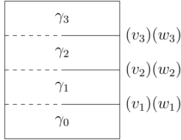
Figure 19: The functor Z : \mathcal{T}_q \rightarrow \mathcal{A} .
