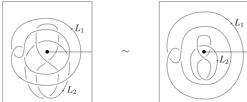
Figure 23: Stacking diagrams.
