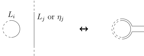
Figure 9: KII move.
