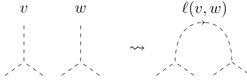
Figure 3: Gluing some legs of a Jacobi diagram with \ell .
