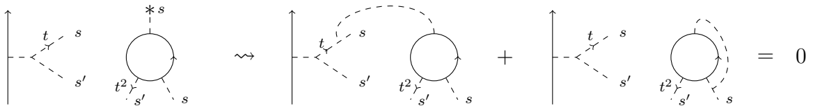
Figure 13: A link relation.
