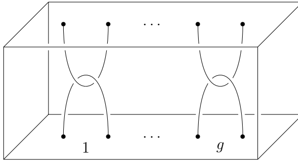
Figure 7: The bottom-top tangle T_g in [-1, 1]^3 .
