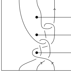
Figure 11: Diagram of a tangle with disks.
