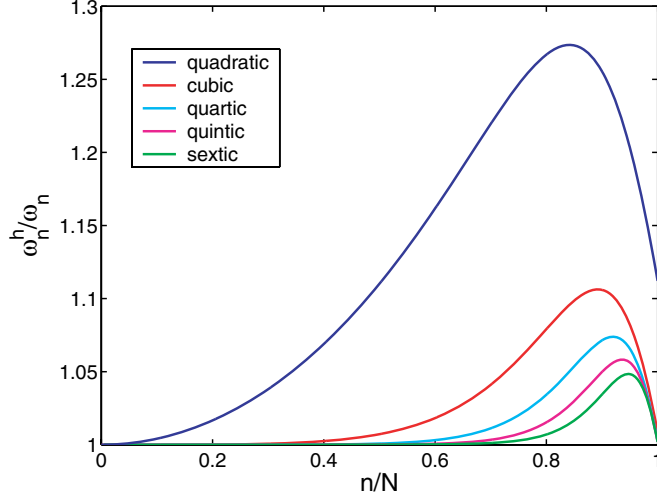
Fig. 27. Simply supported beam. Normalized discrete spectra using equally spaced control points. (These results are identical to those presented in Fig. 21 except the outliers are eliminated.)
