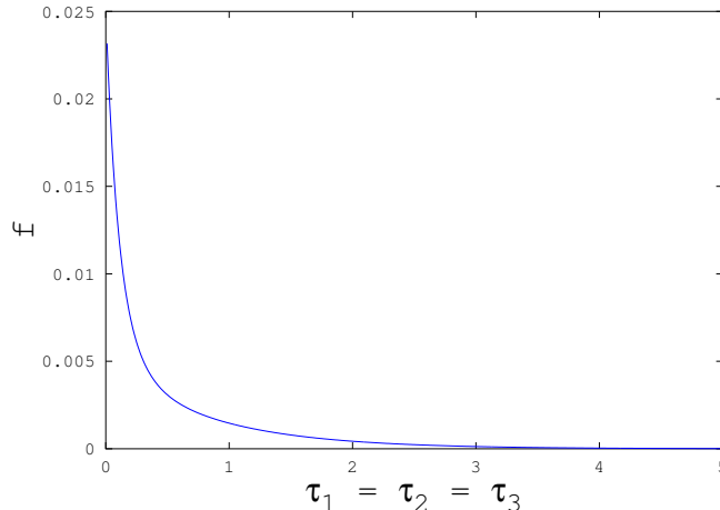
Figure 2: The density f for \tau_1 = \tau_2 = \tau_3
