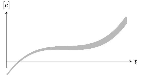
(e) Tube [c](t) = \int_0^t [x](\tau) d\tau
