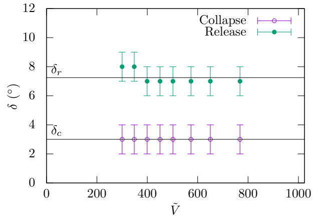
Figure 5: Critical angle for the fibers to collapse \delta_c (hollow circles) when decreasing the tilting angle and to separate \delta_r (filled circles) when the tilting angle is then increased for varying volume of liquid V . The fibers have a radius a = 125 \mu\text{m} , a total length L_{fib} = 87 \text{mm} and a free length L_{free} = 18.6 \text{mm} .
