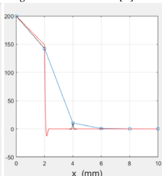
Fig. 26: Solution hom. [1]
