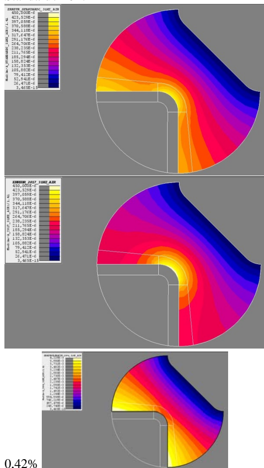
Fig. 52 : 31Hz ( \delta/d=1,97 ) – max=0.045% Standard / 2017
