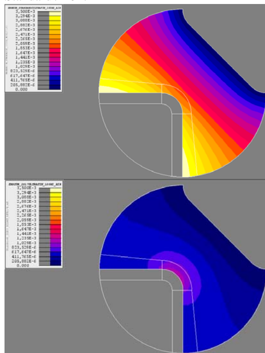
Fig. 54 : 100Hz ( \delta/d=1,095 ) – max=0.35% (0.12%) Standard / 2017
