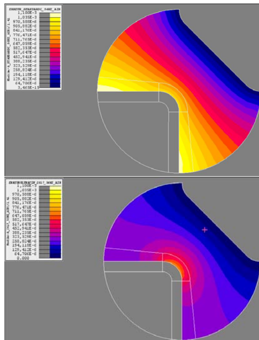
Fig. 53 : 56Hz ( \delta/d=1,46 ) – max=0.11% (0,07%) Standard / 2017
