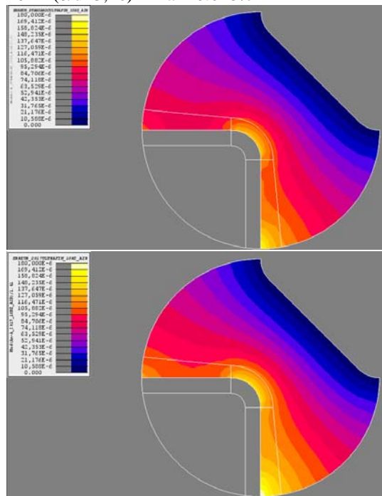
Fig. 52 : 31Hz ( \delta/d=1,97 ) – max=0.045% Standard / 2017
