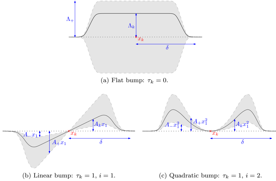
Figure 4: The three shapes of the bump map \Phi_\tau^{\Lambda, \mathbf{A}, i} around a x_k .
