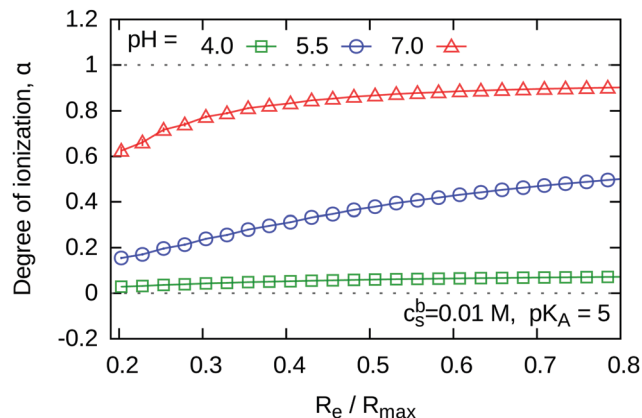
Fig. 6 Degree of ionization of the weak polyelectrolyte gels as a function of chain extension at a fixed salt concentration of c_s^b = 0.01 M and for different pH values.
