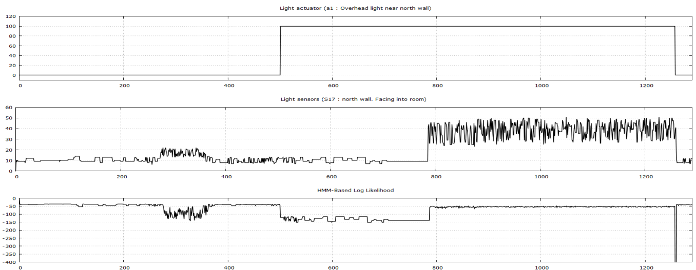
Fig. 18: Results for the computation of the log-likelihood of an observation sequence y_{1:K} (here the luminosity sensor S17 is used) given an input sequence u_{1:K} and the CD-HMM state observer depicted in Fig.11.
