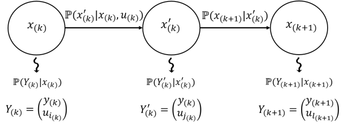
Fig. 10: Considering Moore FSM from a probabilistic point of view leads (1) a transient state x(k) to appear in the HMM state observer and (2) the output vector y(k) to be partitioned with the input vector u(k) ( Y(k) = (y(k), u(k)) ).
