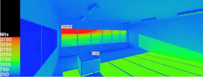
Fig. 4: The distribution of the luminosity in a classroom based on a 3D model [15]
