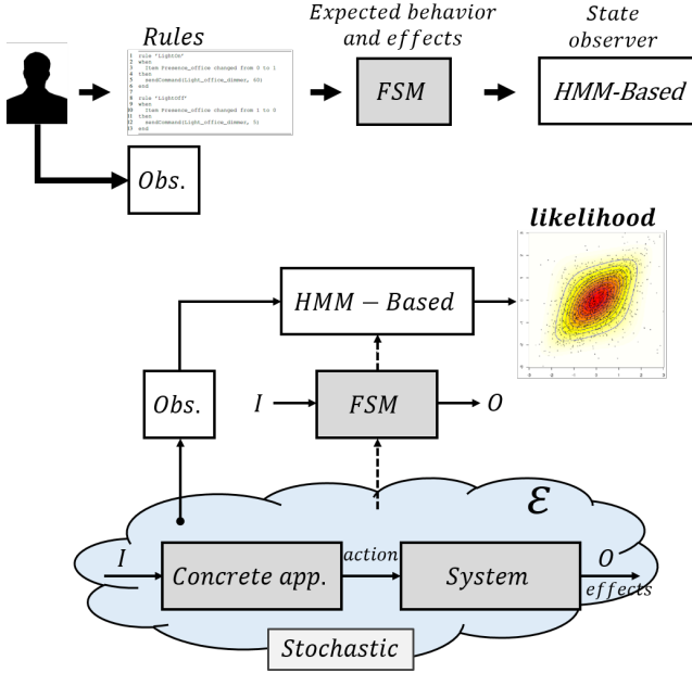
Fig. 8: Approach overview. The model of the ideal expected behavior of an application is specified in terms of the effects it is expected to produce within the physical environment as it executes (Moore FSM). This model is further projected into its probabilistic HMM-Based state observer counterpart. The solution the state observer provides to the hidden state estimation problem through the log-likelihood estimation ( [-\infty, 0] ), can be used to give direct insight into the behavioral conformity of an application interacting with the physical environment.
