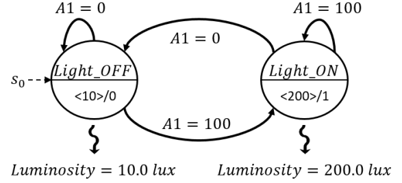
Fig. 6: BAS rules transformed to equivalent Moore FSM
