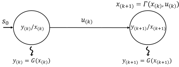
Fig. 5: Moore Finite State Machine (FSM) in a nutshell
