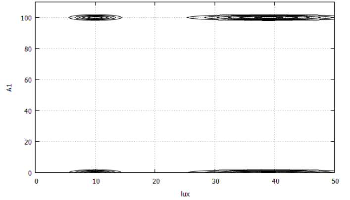
Fig. 12: The parameters of the emission probability functions (matrix B ), expressed as multivariate normal distributions, define viability zones, i.e. zones where the effects of an application within the physical environment are satisfactory without necessarily being perfect. This figure represents the viability zones for all the state emissions defined in Fig.11
