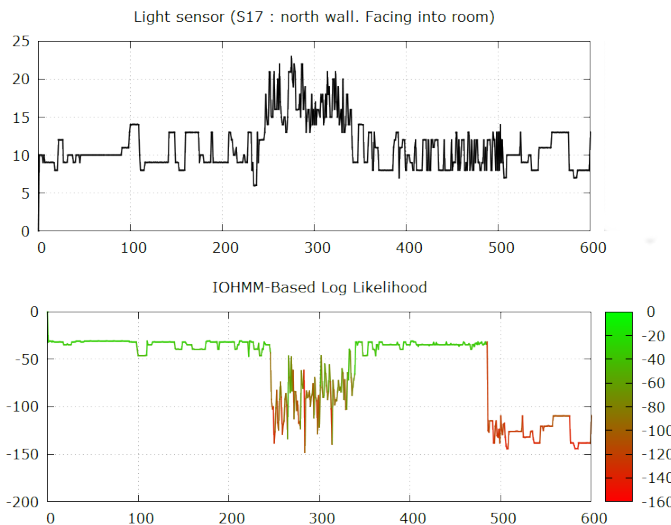
Fig. 19: The CD-IOHMM-based state observer approach, through the log-likelihood ( ]-\infty; 0] ) estimation, allows to quantify, at runtime, the magnitude of the behavioral drift of a concrete application beyond a discrete PASS/FAIL result.
