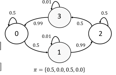
Fig. 11: CD-HMM state observer corresponding to the Moore FSM depicted in Fig.6. We assume that the probability density functions in the matrix B are multivariate normal distributions. Here, the parameter values of the distributions have been populated from the dataset used for the validation of the approach (Section.VI-A).
