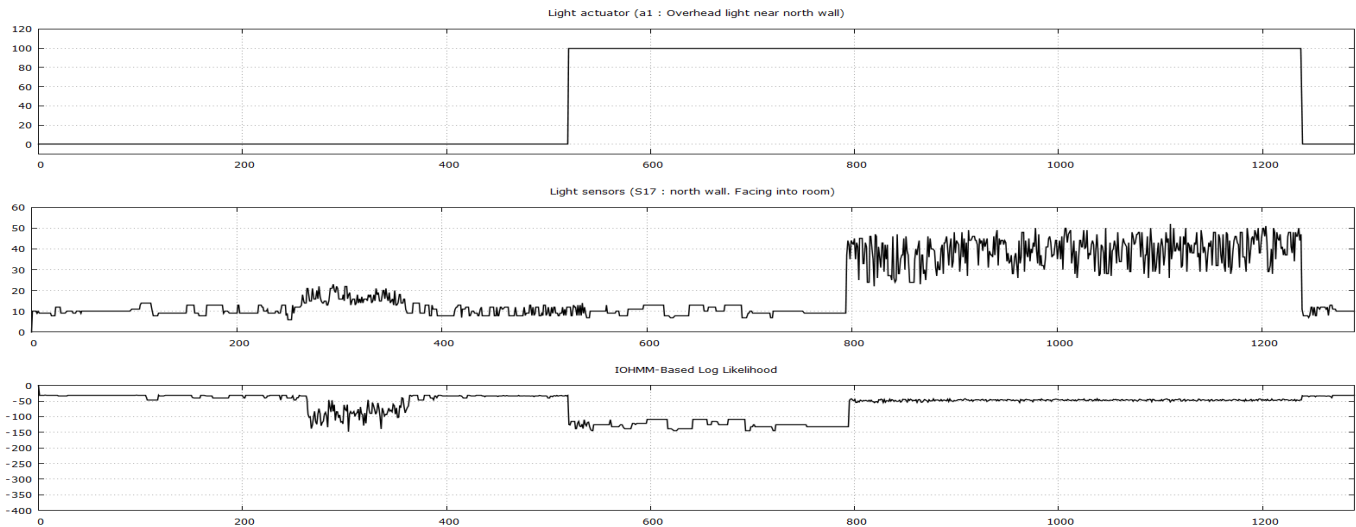
Fig. 17: Results for the computation of the log-likelihood of an observation sequence y_{1:K} (here the luminosity sensor S17 is used) given an input sequence u_{1:K} and the CD-IOHMM state observer depicted in Fig.16.
