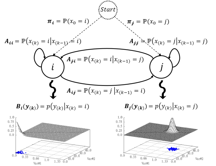
Fig. 7: Multivariate CD-HMM in a nutshell
