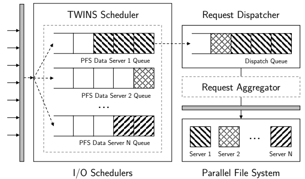
Fig. 2: Flow of requests through the IOFSL I/O node daemon with the new TWINS scheduling option.
