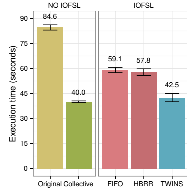
Fig. 6: TWINS vs. collective I/O operations
