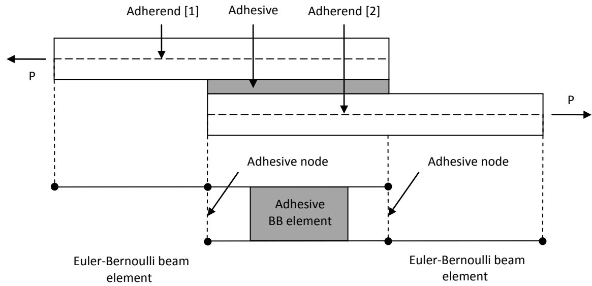
Figure A1-1. Assembly of the single-lap joint configuration. Linear elastic 1D-beam model.
