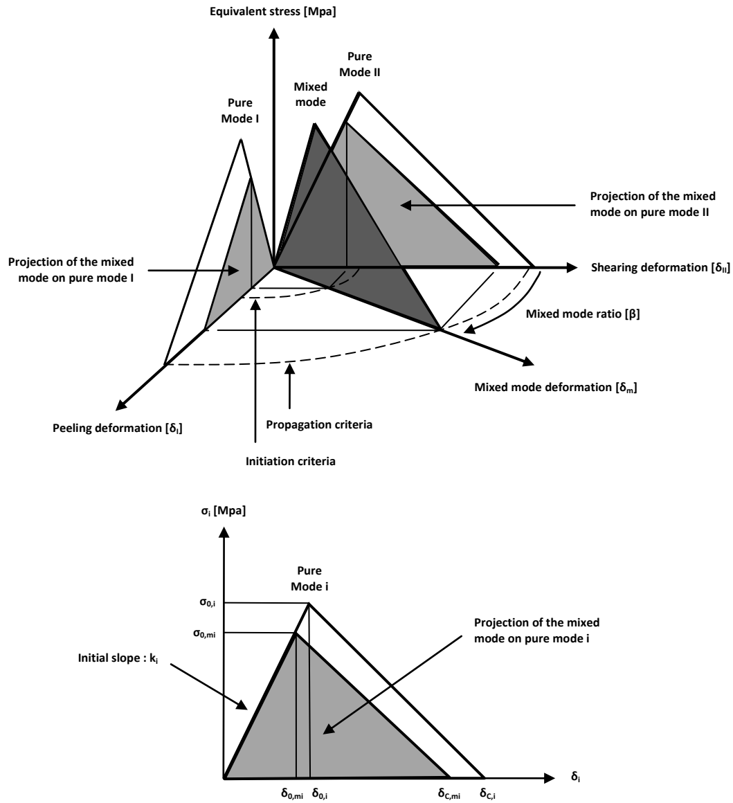
Figure 4. Graphical representation of the mixed-mode parameters. Description of the mixed-mode I/II adhesive behavior.
