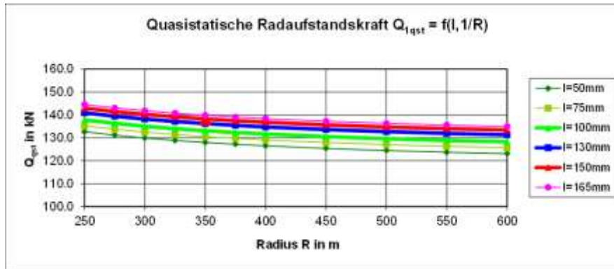
Figure 13: Example for multiple regression analysis of test results for quasi-static track loading parameters
