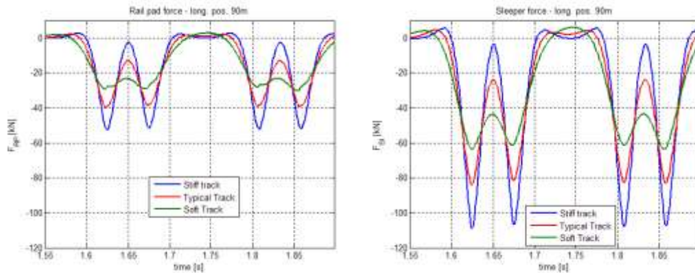
Figure 5 : Vertical forces in the track; rail fastening (left) and ballast (right)
