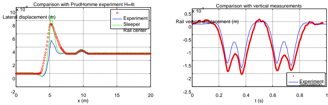
Figure 9: Comparison between simulations and two sorts of experiments
