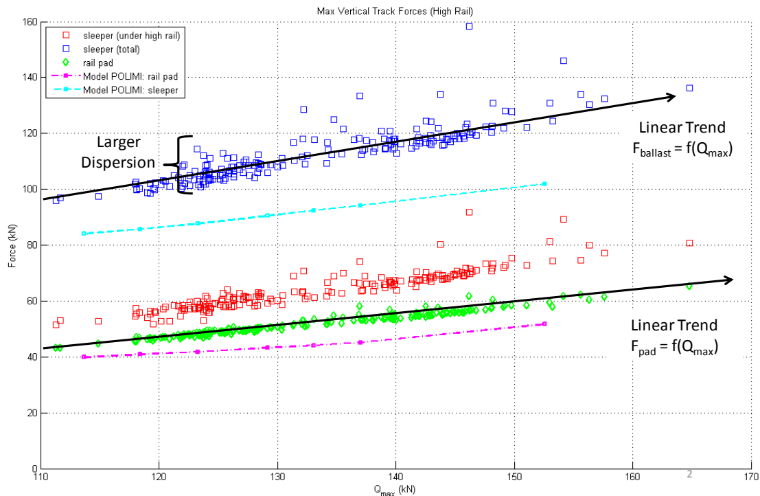
Figure 6: Relationship between track forces (rail pad and sleeper-ballast) and Q_{max}
