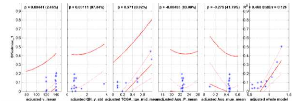
Figure 12: Comparison of \Sigma Y_{max} locomotive regressions on straight track, plots with: speed; track geometry (lateral); equivalent conicity; axleload; wheel-rail friction
