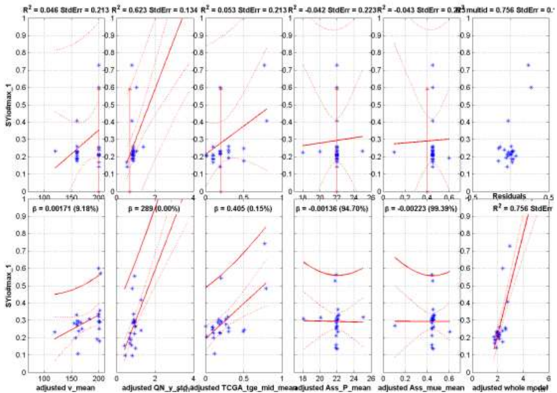
Figure 11: Parameters affecting \sum Y_{max} for the BB26000 locomotive on straight track, plots with: speed; track geometry (lateral); equivalent conicity; axleload; wheel-rail friction
