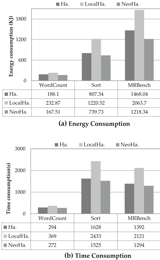
Fig. 5 The comparison of energy consumption and time consumption of WordCount , Sort and MRBench on three systems
