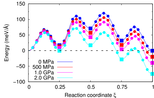
Figure 11. Migration barrier for the \vec{b}_4 disconnection of the \{10\bar{1}1\} twin system under various applied stress. The squares correspond to stable intermediate configurations relaxed independently.
