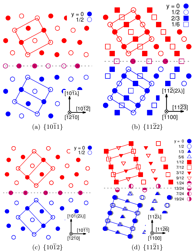
Figure 1. Structures of the relaxed twin boundaries predicted by the EAM potential. The different symbols refer to the depth y of the atoms along the periodicity vector normal to the figure plane. The color refers to atoms of the parent (blue), the twin crystal (red) or the twin plane (purple). (d) For \{11\bar{2}1\} twin system, the grey symbols show the positions of perfectly symmetric twin boundary. The direction perpendicular to the twin boundary z is defined through a factor \lambda = 3/(2\gamma^2) , where \gamma is the c/a ratio of the hcp crystal. 32
