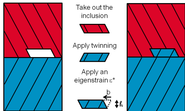
Figure 6. Inclusion model used to calculate the elastic energy of a disconnection dipole.
