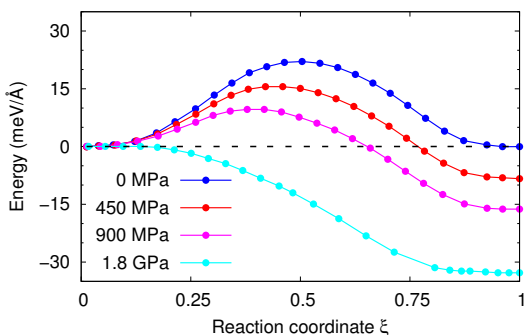
Figure 10. Migration barrier for the \vec{b}_3^S disconnection of the \{11\bar{2}2\} twin system under various applied stresses.
