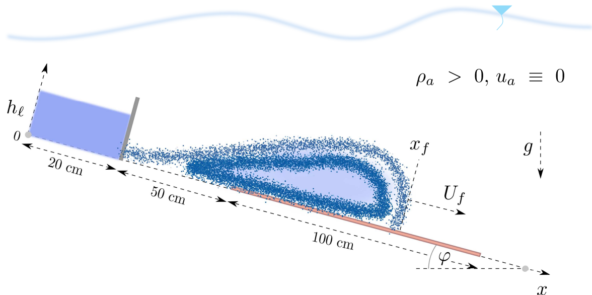
Figure 5. Sketch of numerical lock-exchange experiments.
