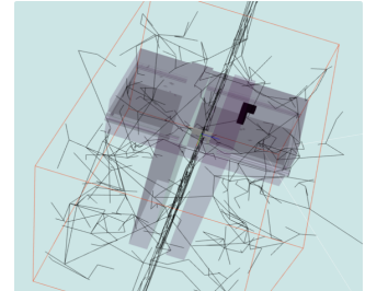
Fig. 17: \alpha = 0.1
