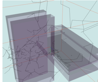
Fig. 16: \alpha = 0
