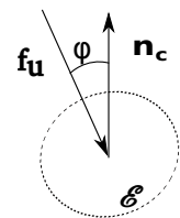
Fig. 2: Small \varphi .
