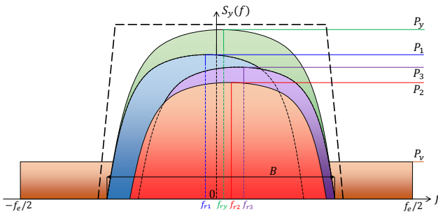
Fig. 4. Representation of the PSDs of the co-channel signals
