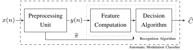
Fig. 1. The common Feature-Based AMC architecture
