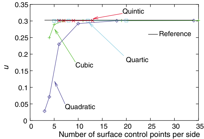
Fig. 44. Shell obstacle course. Scordelis–Lo roof displacement convergence.
