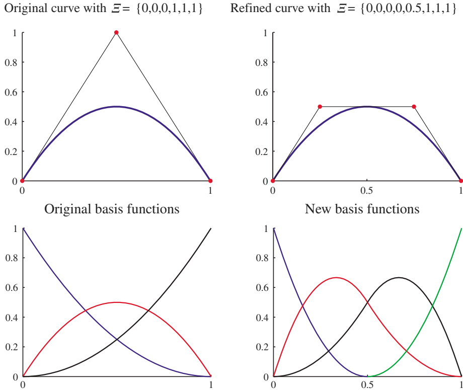
Fig. 8. Knot insertion. Control points are denoted by \bullet .
