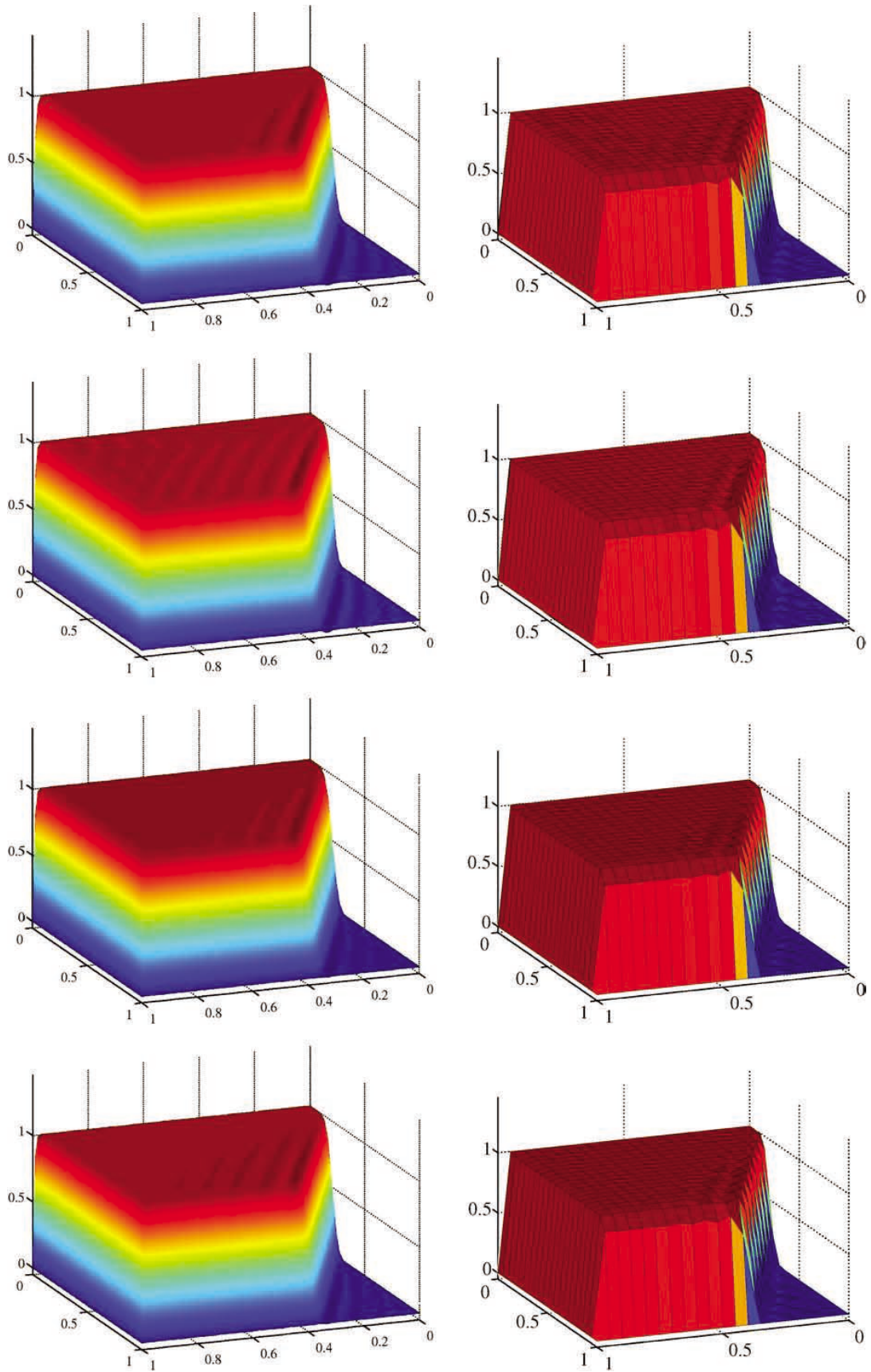
Fig. 71. Advection skewed to the mesh, \theta \approx 63.4^\circ . Top to bottom: results for p = 5 to p = 8 . Left: plot with 100 \times 100 points, Phong shaded. Right: plot with 21 \times 21 points.
