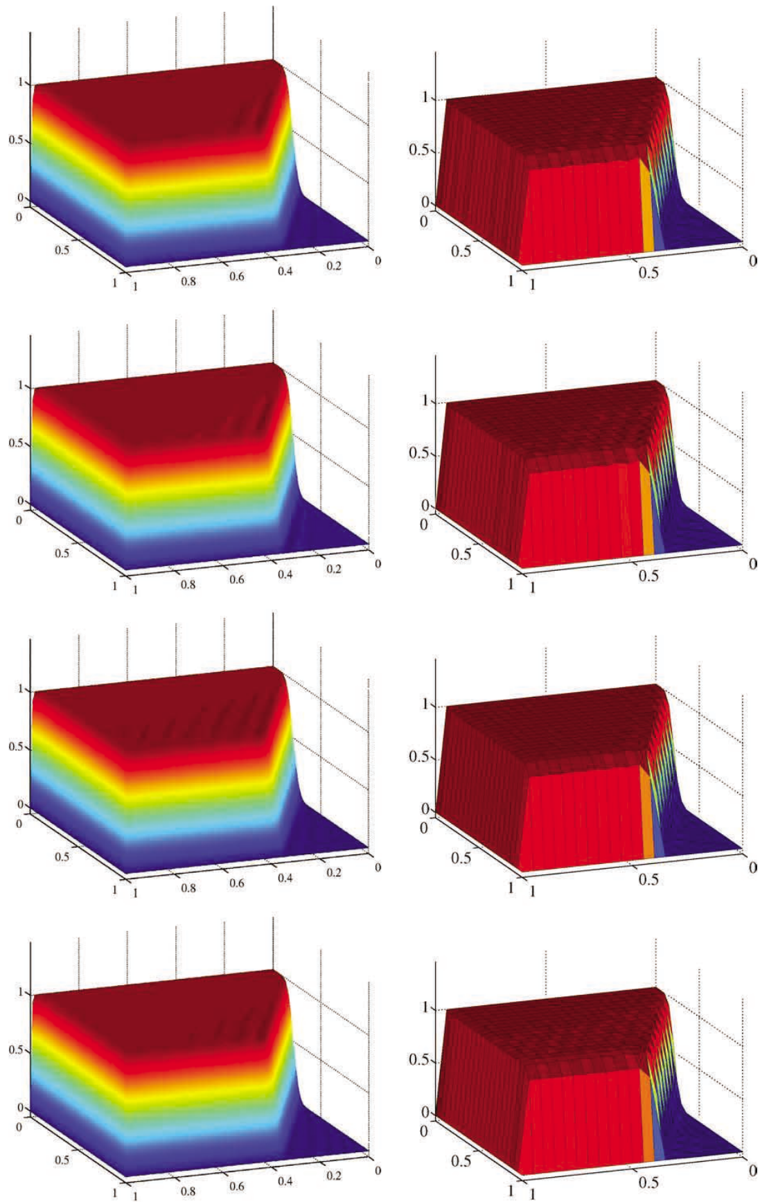
Fig. 72. Advection skewed to the mesh, \theta \approx 63.4^\circ . Top to bottom: results for p = 9 to p = 12 . Left: plot with 100 \times 100 points, Phong shaded. Right: plot with 21 \times 21 points.
