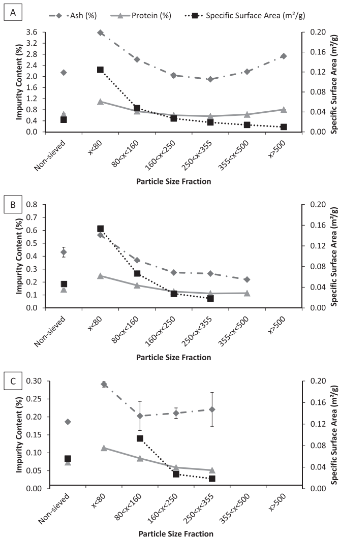
Fig. 2. Impurity content (either protein or ash content; left axis) and specific surface area (right axis) of lactose powders as a function of the particle size class: (A) Wash 0; (B) Wash 1; (C) Wash 2. Results are given as average \pm standard deviation (represented by the error bars). Number of repetitions = 4 for specific surface area, 3 for ash, and 2 for proteins.
