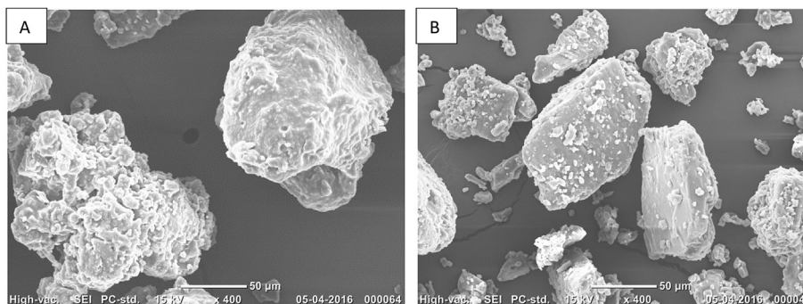
Fig. 3. SEM images showing small particles of different washing grade lactose powders: (A) Wash 0; (B) Wash 2.
