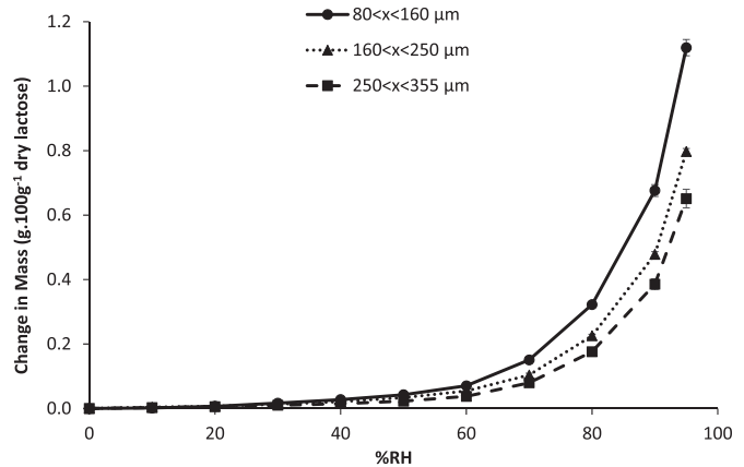
Fig. 4. Moisture sorption isotherms of lactose powder Wash 2 for three different particle size fractions: 80 < x < 160 \mu\text{m} : circles; 160 < x < 250 \mu\text{m} : triangles; 250 < x < 355 \mu\text{m} : squares.
