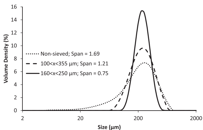
Fig. 6. Particle size distributions of different size fractions (non-sieved, 100 < x < 355 \mu\text{m} and 160 < x < 250 \mu\text{m} ) of lactose powder Wash 0.3.
