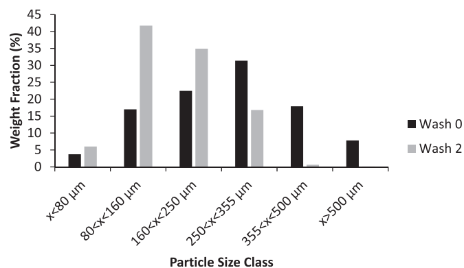
Fig. 1. Particle size distributions of Wash 0 and Wash 2 lactose powders sieved to separate 80, 160, 250, 355 and 500 \mu\text{m} fractions.
