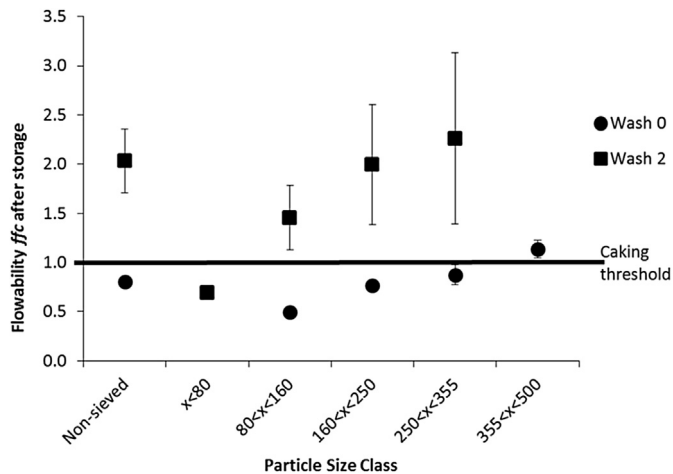
Fig. 5. Flowability ffc of lactose powders Wash 0 (circles) and Wash 2 (squares) as a function of particle size class after storage for four days at 60% RH and 20 °C and under a consolidation stress of 9.3 kPa.
