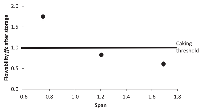
Fig. 7. Flowability ffc of different size fractions of lactose powder Wash 0.3 as a function of the span of the particle size distribution. The size fractions were 160 < x < 250 \mu\text{m} , 100 < x < 355 \mu\text{m} and non-sieved, with the span being 0.75, 1.21 and 1.69 respectively. The measured d 50 were 249 \mu\text{m} , 249 \mu\text{m} and 230 \mu\text{m} respectively. The ffc was measured after storage for four days at 60% RH and 20^\circ\text{C} and under a consolidation stress of 9.3 kPa.
