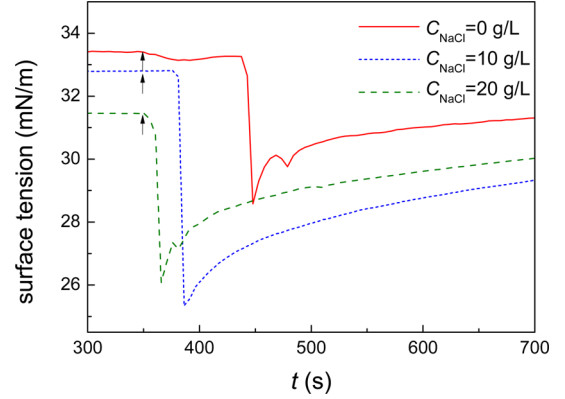
Figure 5. Time evolution of the surface tension of an aqueous phase upon injection below the air/aqueous phase interface of oil droplets dispersed in the same aqueous phase. The aqueous phase contains SDS at a concentration C_{\text{SDS}} = 2.5 g/L and different \text{NaCl} concentrations as indicated in the legend. The black arrows indicate the time of injection.
