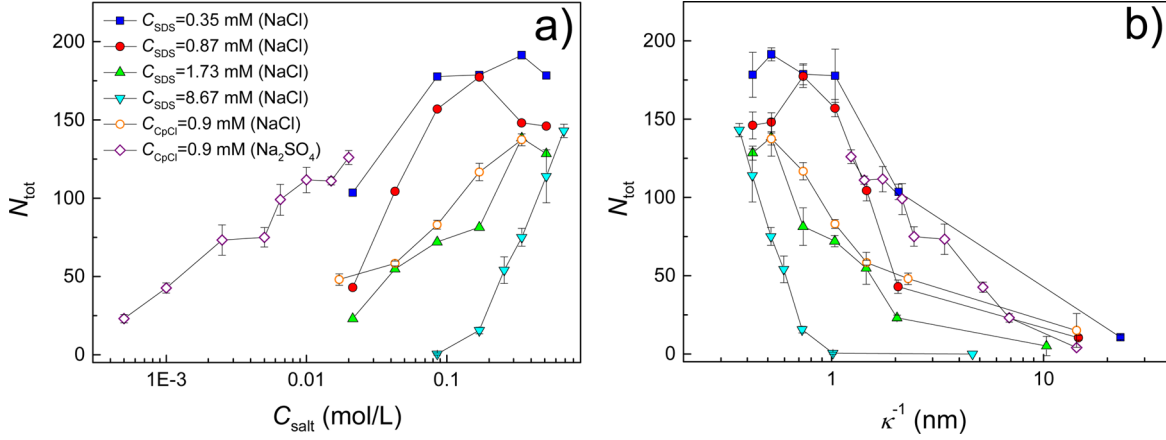
Figure 3. (a) Evolution of the total number of perforation events, N_{\text{tot}} , with the salt (NaCl and \text{Na}_2\text{SO}_4 ) concentration of the aqueous phase of emulsions stabilized by anionic (SDS) or cationic (CpCl) surfactants. (b) Same data as in (a) but plotted as a function of the Debye length of the aqueous phase \kappa^{-1} .
