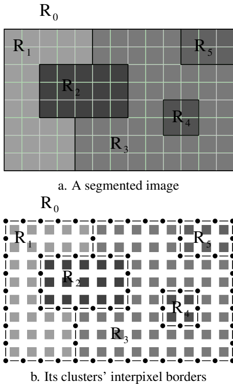
Figure 2: Interpixel Vision
