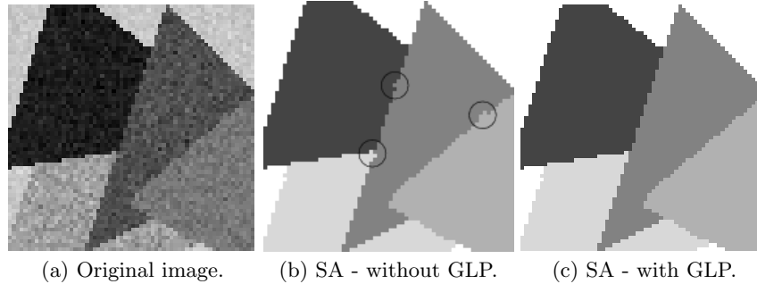
(a) Original image. (b) SA - without GLP. (c) SA - with GLP.
