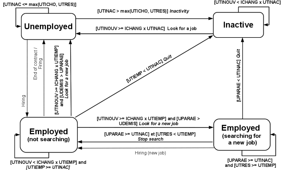
Figure 4: State diagram describing the main transitions of individuals and their decision-making process. Each utility is calculated according to the equation 9. Legend: UTINAC : utility to be inactive. UTINOUV : utility of a new job, estimated through prospecting. UTICHO : utility to be unemployed. UTRES : utility of reservation. UOTJS : utility of the OTJS (On-the-Job-Search) state. UTIEMP : utility to be employed. UDEMIS : utility to quit. ICHANG psychological cost to change state (calibrated exogenous parameter). Dotted arrows represent decisions that do not fully depend on the agent (i.e. taken by the firm.)
