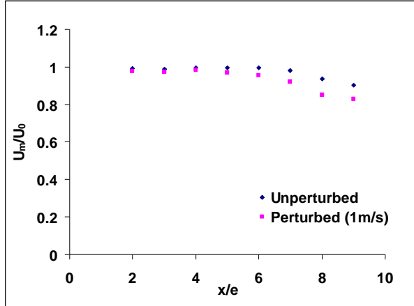
Figure 5 Decay rate of the streamwise velocity
