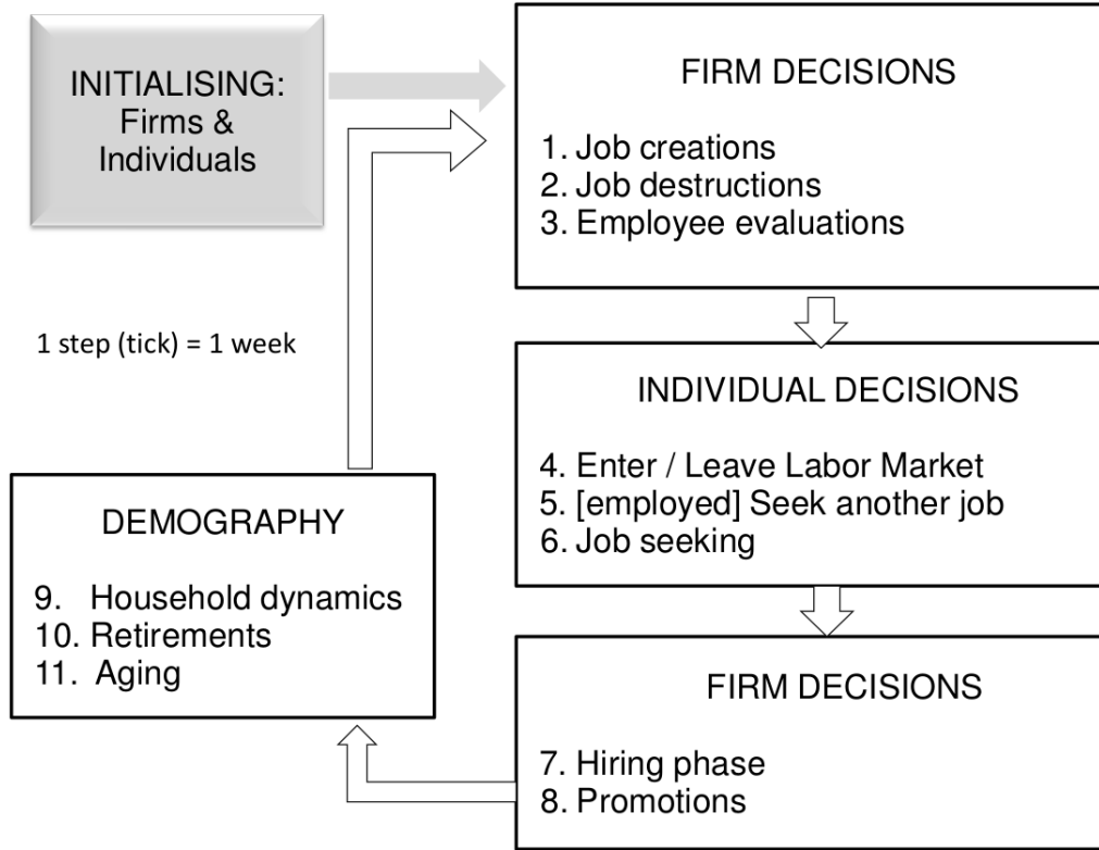
Figure 1: The simulation cycle in WorkSim
