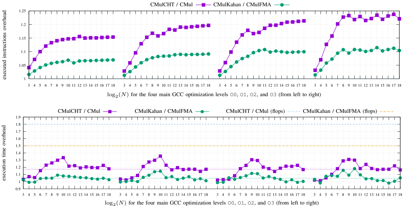
Fig. 1. Overheads in terms of numbers of executed instructions and execution time implied by CMULCHT and CMULKAHAN in double precision on a Cortex-A57 processor (for the four main optimization levels of GCC and for FFT of size N \in \{2^3, 2^4, \dots, 2^{18}\} ). In the bottom figure, dotted horizontal lines show the average values of execution time overheads, and dashed horizontal lines show the theoretical arithmetic cost overheads.
