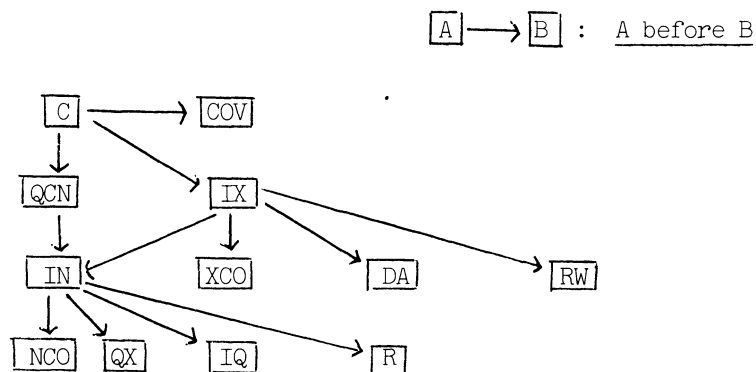
Fig. 3. Loading strategy for the CCDN data base
