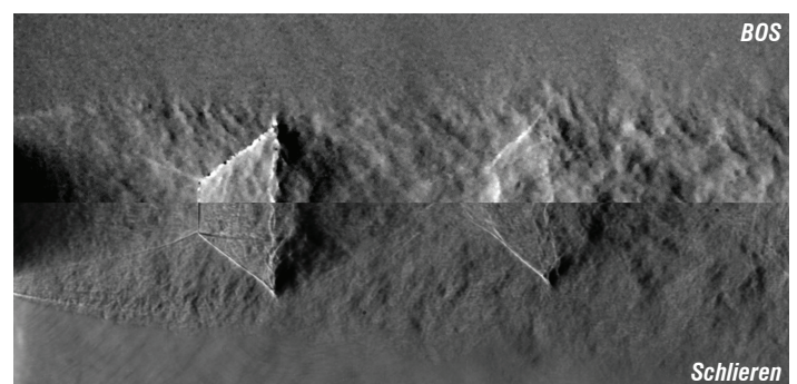
Figure 13 – Experimental images of an under-expanded jet with \text{NPR} = 5 . With a careful choice of the experimental conditions, the BOS deviation image (top half-image) exhibits a spatial resolution comparable to that of traditional Schlieren (bottom half-image)
