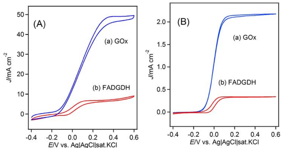
Fig. 5. Rotating disk cyclic voltammograms in 0.1 M phosphate buffer containing 0.5 M glucose, at pH 7.0, 37 °C, 8000 rpm, and 20 mV s -1 for polymer II-based electrodes. Glucose oxidation by GOx (blue curve (a)) and d-FADGDH (red curve (b)). The total hydrogel loading was 1000 μg cm -2 and the polymer:enzyme:crosslinker ratio was 45:45:10 for polymer I and polymer II. (For interpretation of the references to color in this figure legend, the reader is referred to the web version of this article.)
