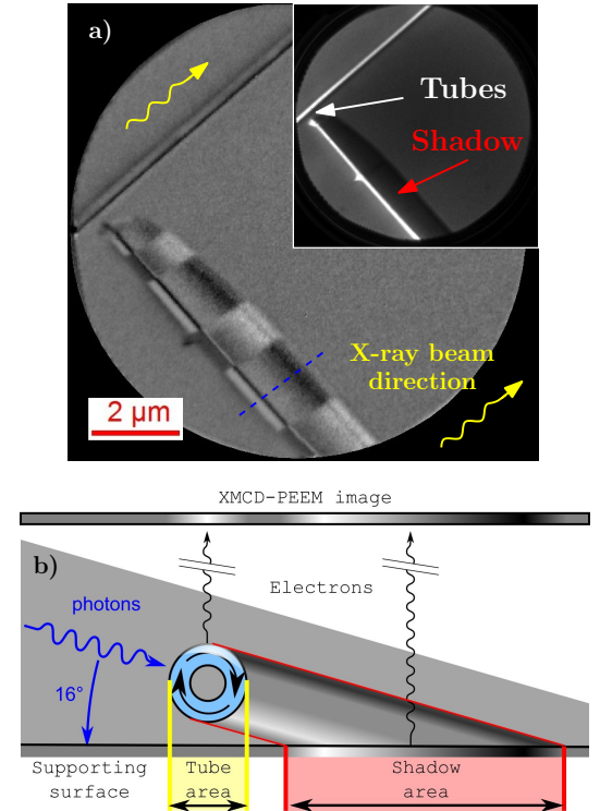
Fig. 2. Magnetic orthoradial flux-closure domains. a) XMCD-PEEM (Co- L_3 edge) image of two orthogonal tubes. The tube along the beam (top) gives rise to almost zero contrast, whereas strong contrast is observed for the tube perpendicular to the beam, revealing domains with orthoradial magnetization. The grey line in the shadow close to the rim comes from oxidation of the inner tube surface (nonmagnetic). The inset shows a non-magnetic photoemission electron microscopy image of the tubes. b) Scheme with the orthoradial magnetization and XMCD-PEEM contrast corresponding to a line profile of an orthoradial domain marked by a blue, dashed line in a). Note that in the experiment the tubes lie on the substrate and only part of the shadow can be observed; further the scheme is valid only for L_3 edges of 3d metals. Sometimes contrast inversion can be seen also in the tube area as detailed in[28].
