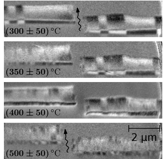
Fig. 5. Changing the magnetic anisotropy upon gradual annealing of the tubes. XMCD-PEEM images (same contrast range [-13\%..13\%] ) of the same tubes after annealing at increasing temperature. All images are taken after cooling down to room temperature. X-ray beam arrives close to perpendicular to the tube axis as indicated by the arrow. With the increasing annealing temperature, the orthoradial magnetization pattern becomes weaker and gradually disappears, persisting only close to the tube extremity (end curling). The degree of the transformation is not the same for both tubes, probably due to a different tube wall thickness. After remagnetization along the tube axis (bottom image), both tubes display close to uniform contrast in the shadow, a sign of magnetization pointing along the tube axis. The contrast (bottom image) is weak due to a very small component of the magnetization along the beam.
