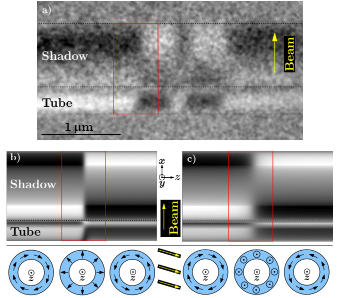
Fig. 4. Domain walls between flux-closure domains. a) Experimental XMCD-PEEM with the beam perpendicular to the tube featuring 5 orthoradial domains, the red rectangle highlights an area with one domain wall. We compare this DW to a simulated contrast for b) Bloch and c) Néel walls. Schematic tube cross-sections below the simulations show the magnetization in domains and the domain wall (in the middle of the tube) respectively. Note that in the experiment part of the shadow is covered by the structure itself.
