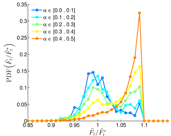
FIG. 7. Probability distribution function of the ratio \tilde{F}_t/\tilde{F}_t^* for the sliders that moved upon inclination – The data are from the 20 same numerical runs as in Fig. 6 [ N = 100 , \xi = 0 , \tilde{l} = 10 , \mu_d = 0.55 , \bar{\mu}_s = 0.6 , and \sigma_\mu = 0.01 ].
