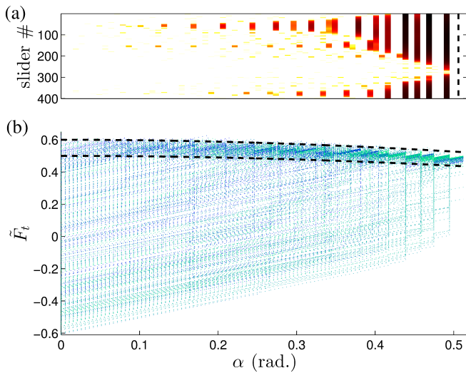
FIG. 4. Behavior of a large system with global coupling upon inclination – (a) Hot map of the displacements \Delta\tilde{x}_i vs. angle \alpha . (b) Tangential force \tilde{F}_t vs. angle \alpha (The slider number is indicated by the color bar). The upper dashed line is the stability limit: \bar{\mu}_s \cos \alpha . The lower dashed line is the arrest limit (2\mu_d - \bar{\mu}_s) \cos \alpha [ N = 10 , \xi = 0.001 , l = 10 , \mu_d = 0.55 , \bar{\mu}_s = 0.6 , and \sigma_\mu = 0.01 ].
