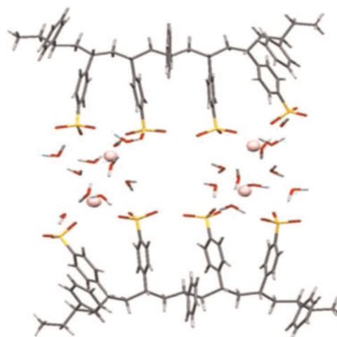
Fig. 9. Optimized geometry of macromolecular model formed by two polymer fragments equilibrated by Ca^{2+} .
