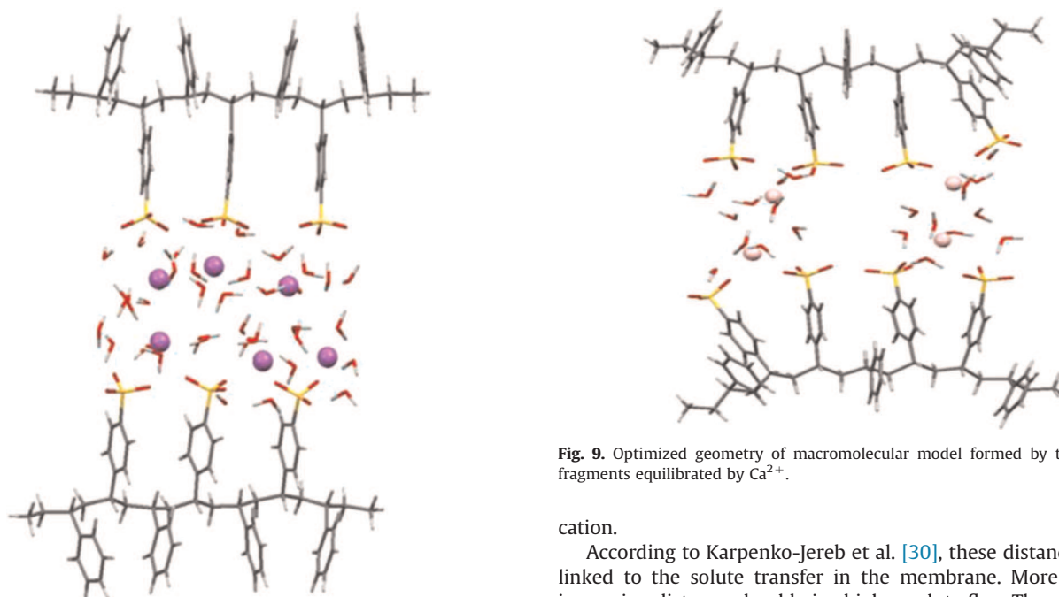
Fig. 8. Optimized geometry of macromolecular model formed by two polymer fragments equilibrated by Na^+ .
