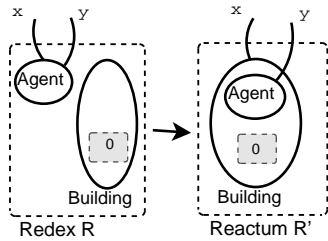
Figure 2: A reaction rule
