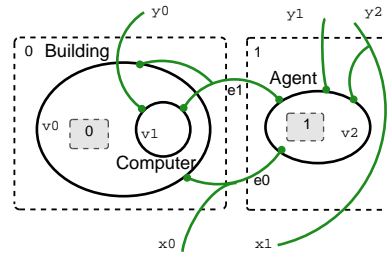
Figure 1: A Bigraph G
