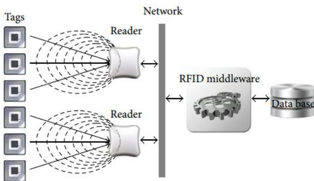
Figure 1. RFID System components.
