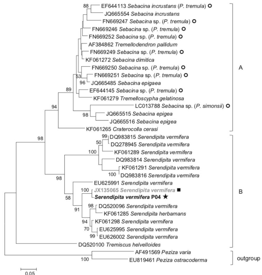
Fig.2 MaximumLikelihood phylogenetic tree based on rDNA ITS sequence data from Sebaciniales identified by ITS- RLFP analysis (square) or from pure-cultured isolated strains (star) with known and selected fungal species from GenBank with high sequence similarities. GenBank Sebaciniales sequences arising from ECM poplar roots are denoted by open circles. Bootstrap values over 50 % (1000 replicates) are indicated above the branches. The two Sebaciniales clades (A & B) described by Riess et al. (2014) are represented.
