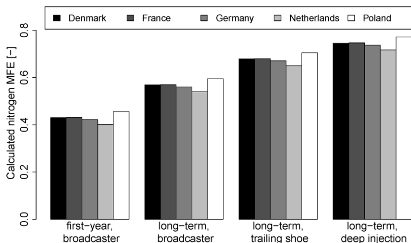
Figure 1. Calculated nitrogen MFE values for different application methods and geographical locations
