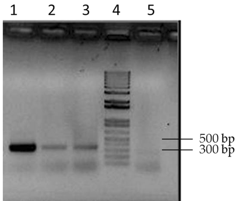
Fig. 4 Agarose gel electrophoresis of msp5 gene amplification. 1 % agarose. Lane 1: positive control; Lane 2: anteater sample; Lane 3: taruca sample; Lane 4: Molecular marker (1 Kb plus); Lane 5: negative control
