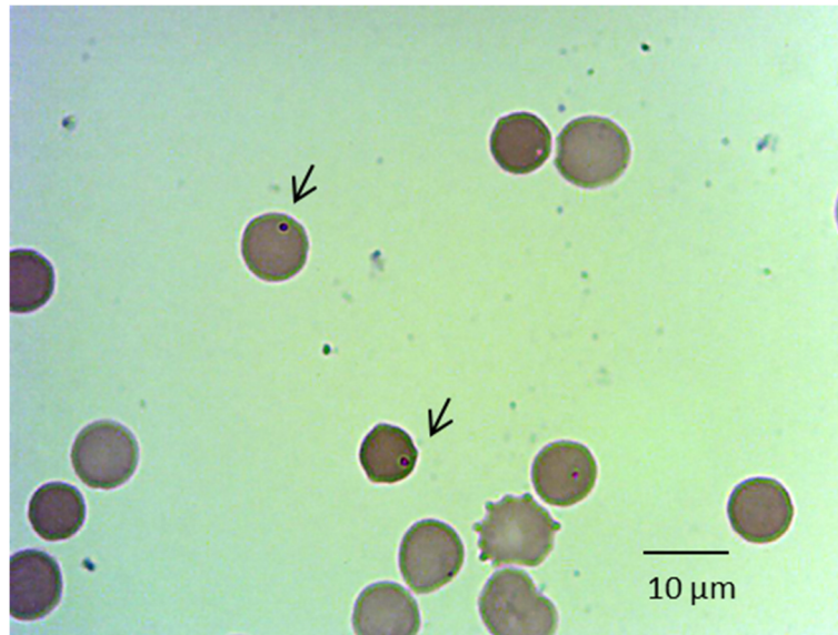
Fig. 2 Blood smear from Myrmecophaga tridactyla . The arrows point out spherical inclusions suggestive of A. marginale . May Grunwald-Giemsa, 100x oil immersion
