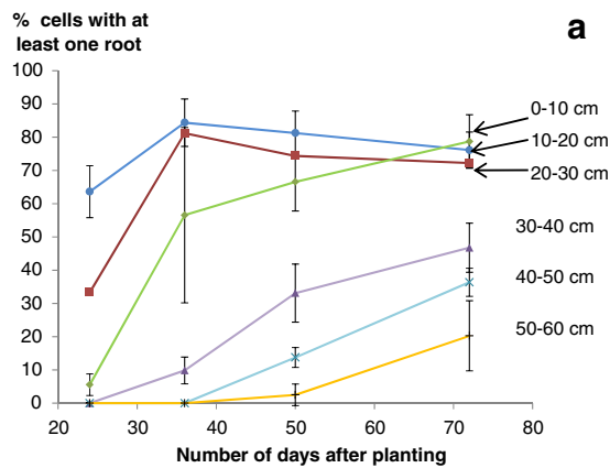
Fig. 3 Soil exploration by the pepper roots in Alénia station. The data indicate the percentage of 2 \times 2 -cm cells of each layer containing at least one root. The means \pm standard error of 15 data per treatment are shown. a The soil exploration by pepper roots is presented for each soil layer of 10-cm depth from the surface, in 2013, for plants cropped at a density of
