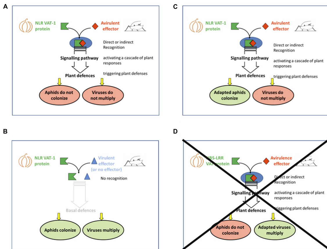
FIGURE 3 | Models of A. gossypii /Vat-melon plant interaction based on interaction (direct or not) between the VAT protein and the avirulence effector (Boissot et al., 2016). The three cases observed were: (A) resistance to aphids and viruses, (B) susceptibility to aphids and viruses, (C) susceptibility to aphids and resistance to viruses. (D) A fourth outcome, resistance to aphids and susceptibility to viruses, was not observed.
