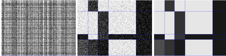
FIG 1. A binary data matrix before (left) and after (middle) row and column reordering, and its parsimonious data representation (right).
