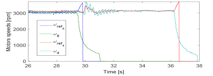
Fig. 10. Motors speeds and their references [rpm] during hovering flight when injecting total failures on motors 4 and 8.
