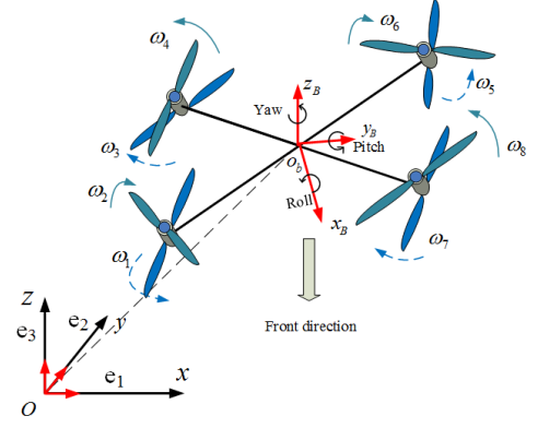
Fig. 1. Inertial and Body-Fixed Frames
